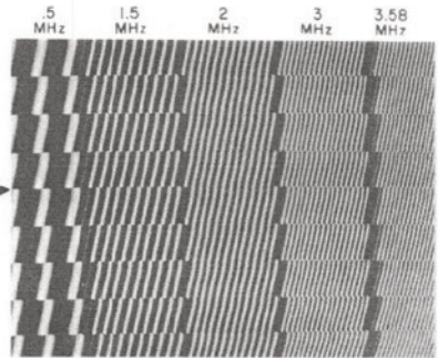
Figure 16—Jogs in Bar Pattern, Insufficient Head Penetration
