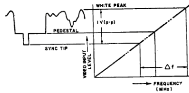
Fig. 4. Video-FM characteristic.
