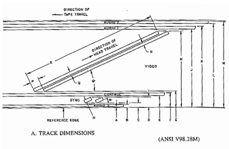
The track configuration for 1-inch type A tapes (Ampex: 1966, p. 2).
