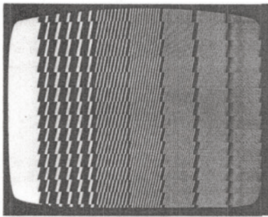
Figure 16—Jogs in Bar Pattern, Insufficient Head Penetration
