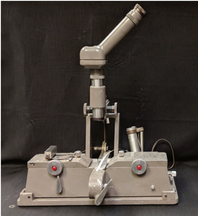
Figure 16. Block or jig of the type used to splice 2-inch tapes. 31
