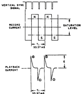
Fig. 5. Control signal waveforms.
