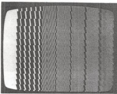
Figure 17—Jogs in Bar Pattern, Excessive Head Penetration
