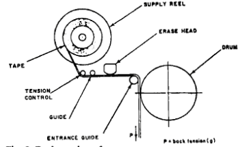
Fig. 9. Back tension of tape.
