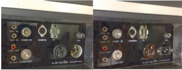
C.3 Figure 7. Sony AV 3/8650 back connector panel before and after connector upgrades.
