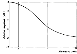
Fig. 6. Video de-emphasis curve.
