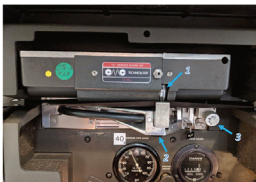
Figure 13. The head assembly on an Ampex model MK XV. Arrow 1 points to the head wheel. Arrow 2 points to the scallop adjustment; see figure 14 for an example of scalloping error. Arrow 3 points to the tip penetration adjustment.
