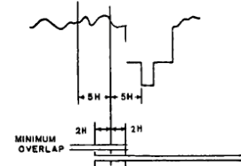
Fig. 7. Switching position of two video heads and the overlap.
