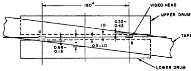
Fig. 2. Drum, video head and tape position.
