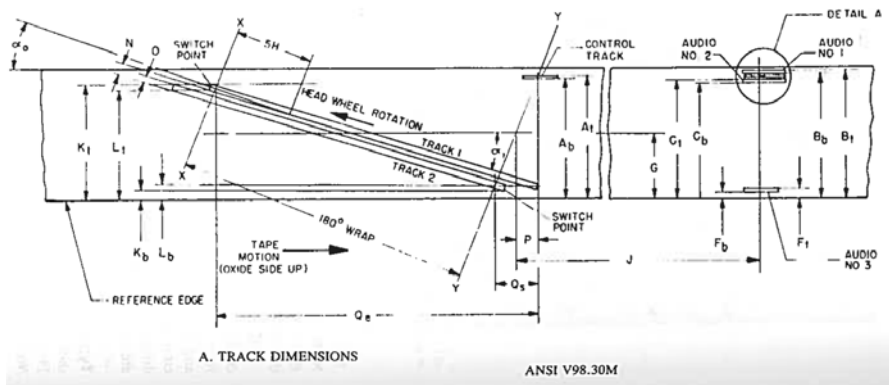
C.4 Figure 2. 1-inch type C track configuration
