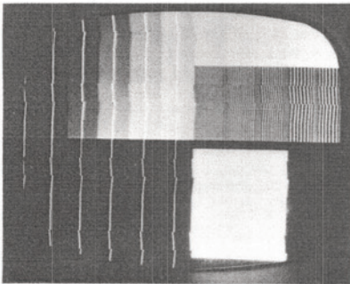
Figure 14—Steps in Bar Pattern (Quadrature Misadjusted)
