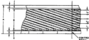
Fig. 2. Drum, video head and tape position.
