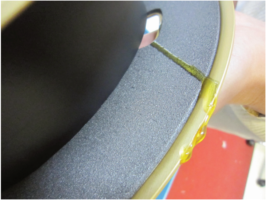
Figure 3. Quad reel showing foam flange and failing glue.
