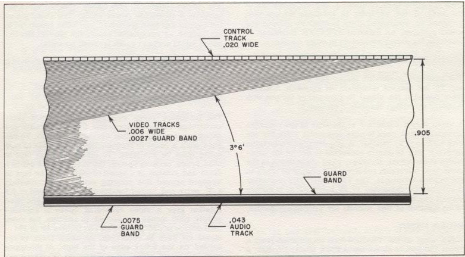
The track configuration for 1-inch type A tapes (Ampex: 1966, p. 2).
