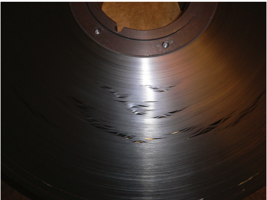
Figure 5. Examples of poor tape pack and its effects on the tape. The first image depicts an example of wrinkled red oxide tape; in addition to the wrinkling, the oxide has come off the bottom edge of the tape.
