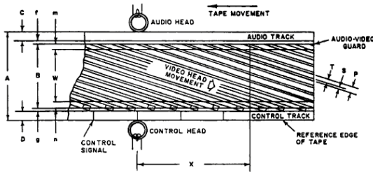
Fig. 1. Magnetic tape pattern (tape seen from magneto-sensitive surface).
