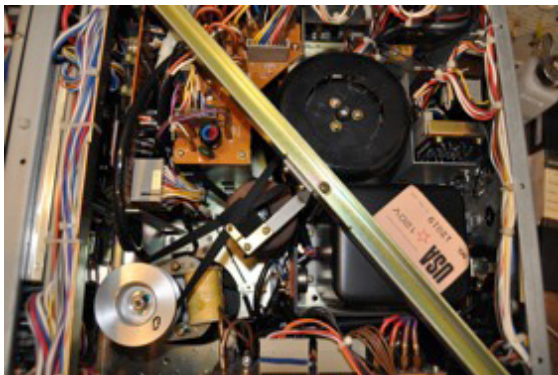
C.3 Figure 4. Internal view of 1/2-inch VTR, showing pulley and drive belt.
