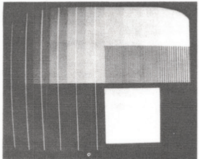
Figure 15—Normal Appearance of Alignment Tape Playback
