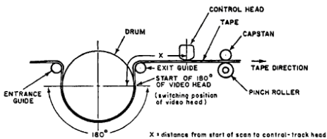
Fig. 8. Position of audio and control head.
